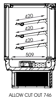
SECTION VIEW
