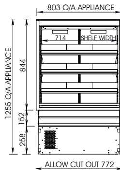
FRONT ELEVATION
