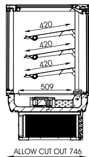
SECTION VIEW
