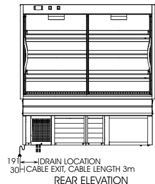
REAR ELEVATION
