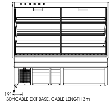
REAR ELEVATION
