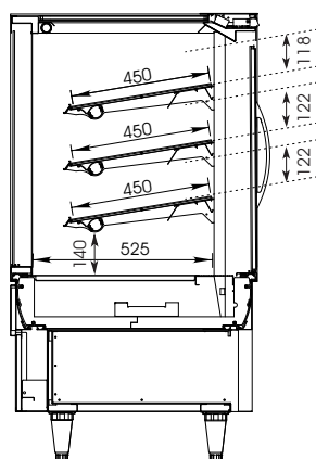
SECTION VIEW
